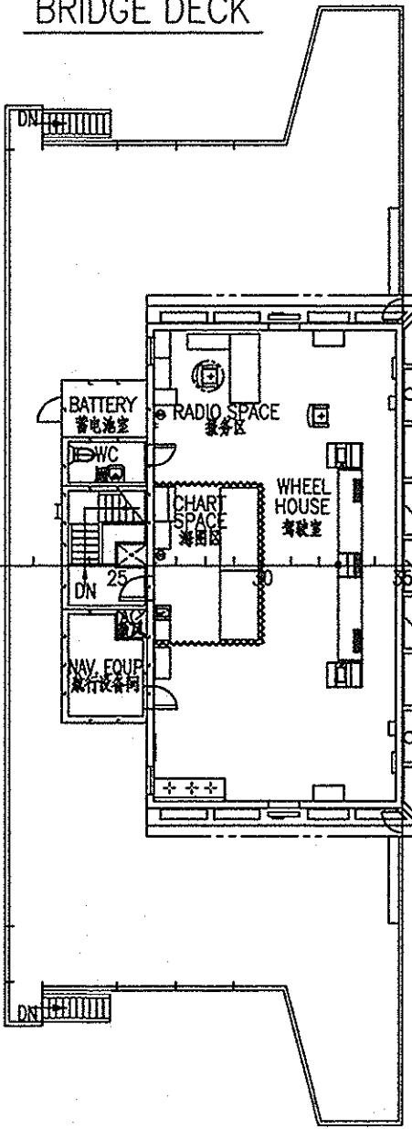
桥楼甲板 BRIDGE DECK
