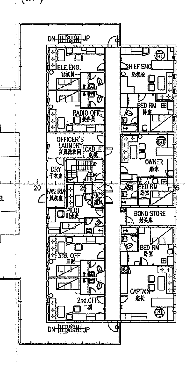
C甲板 C DECK (8P)
